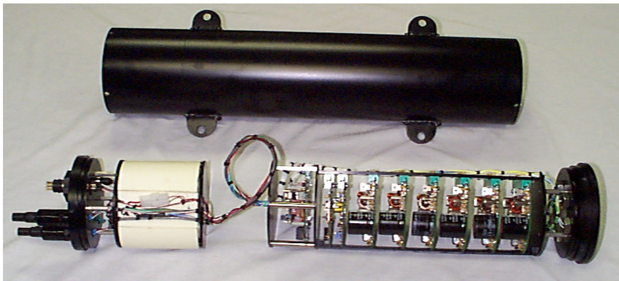
Figure 3. TAPS-6 removed from pressure case. The connector endcap is on the left; attached to it is the battery (white cylinder). The transducer endcap is on the right; attached to it is the electronics card cage. The six cards closest to the transducer are the acoustic transceivers. Next are the instrument I/O card and the power control card. The stacked card in a separate section of the card cage is the CPU card.
