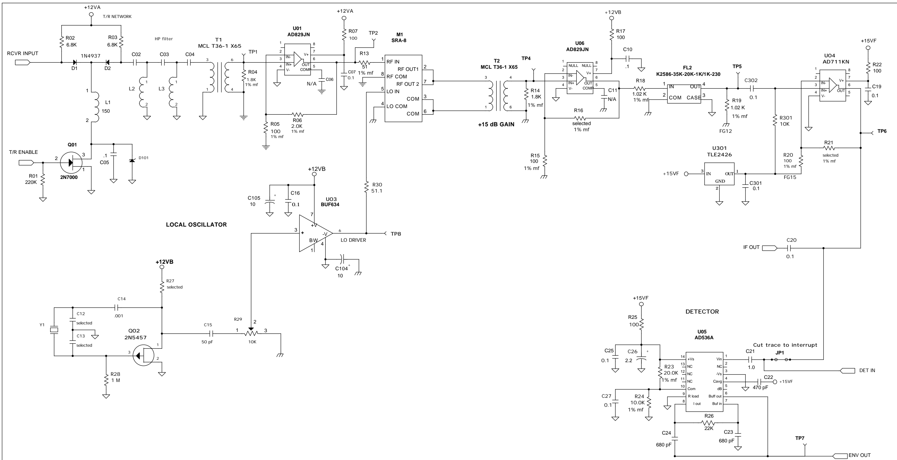
TRANSCEIVER V - rev 4 28 Nov 1997 Receiver section
