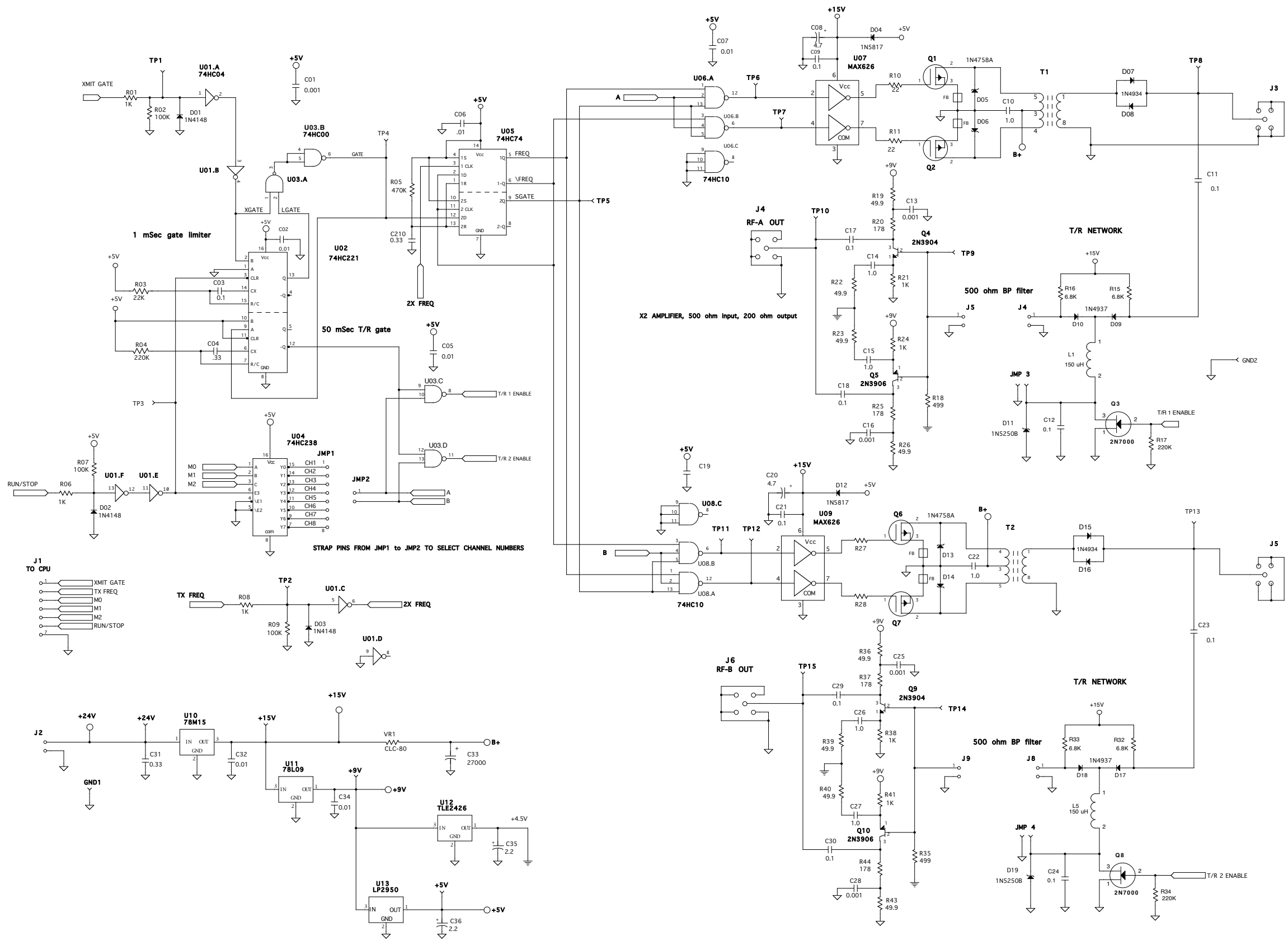
TAPS NEW GENERATION DUAL TRANSMITTER Rev 1: 04 May 2012
